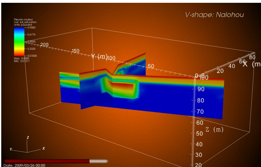
Saturation, ParFlow-CLM
